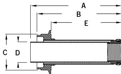
MALE LINDE TYPE HYDROGEN SERVICE*
