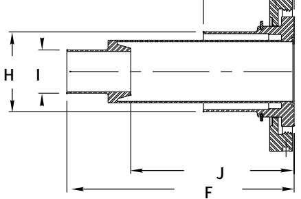
FEMALE AIR FORCE HYDROGEN SERVICE
