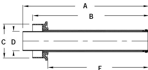
MALE HELIUM SERVICE*
