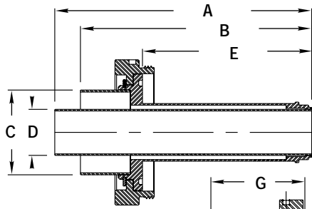
MALE AIR FORCE HYDROGEN SERVICE *
