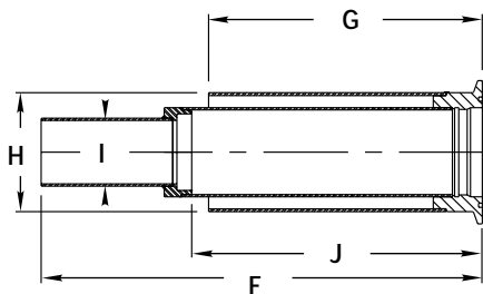
FEMALE LINDE TYPE HYDROGEN SERVICE*
