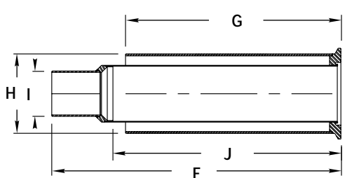
FEMALE HELIUM SERVICE*
